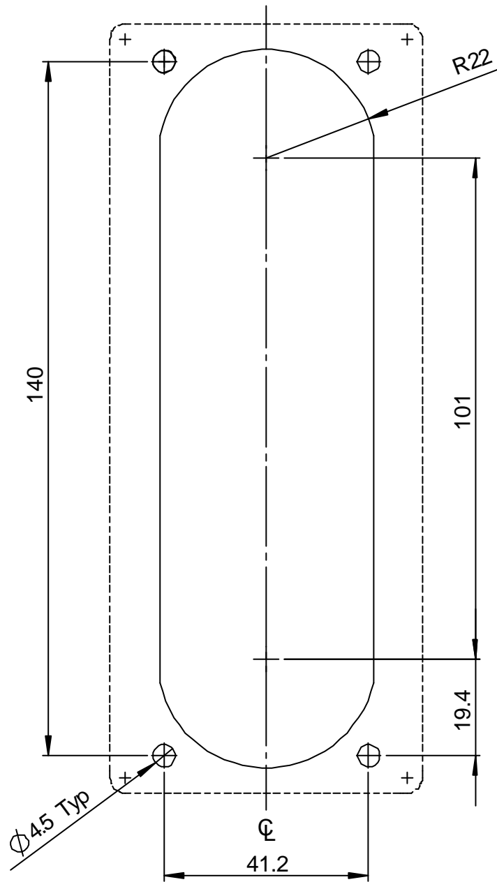
VIEW FROM FRONT OF PANEL
